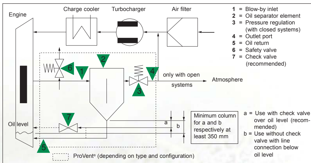
Fig. 2: Diagram of closed and open crankcase ventilation
